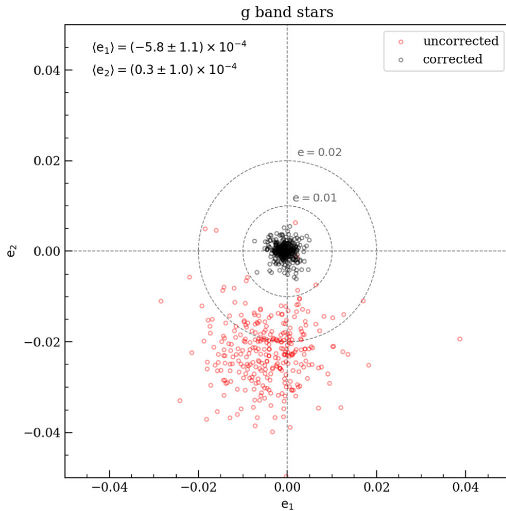
Figure 1. from Eunmo Ahn et al 2024 Astrophys. J. 973 doi:10.3847/1538-4357/ad65dc https://dx.doi.org/10.3847/1538-4357/ad65dc © 2024. The Author(s). Published by the American Astronomical Society.
