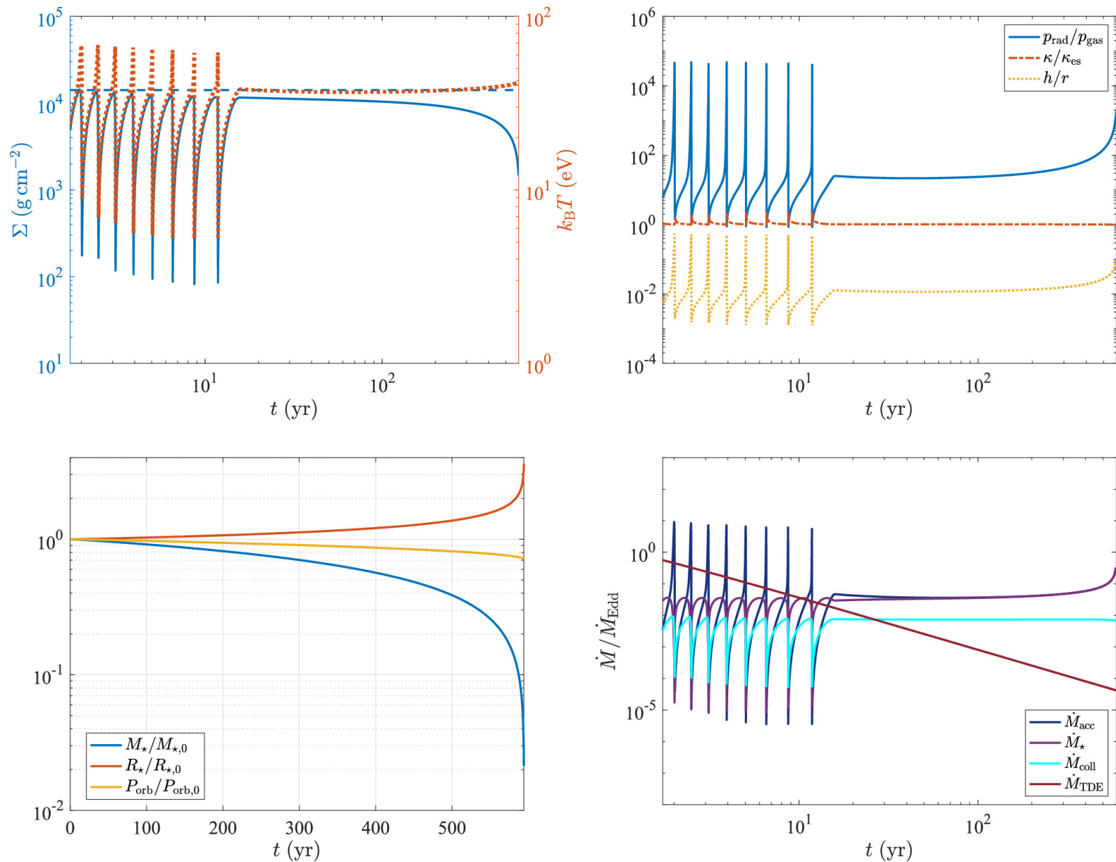
Figure 5. from Itai Linial and Brian D. Metzger 2024 Astrophys. J. 973 doi:10.3847/1538-4357/ad639e https://dx.doi.org/10.3847/1538-4357/ad639e © 2024. The Author(s). Published by the American Astronomical Society.
