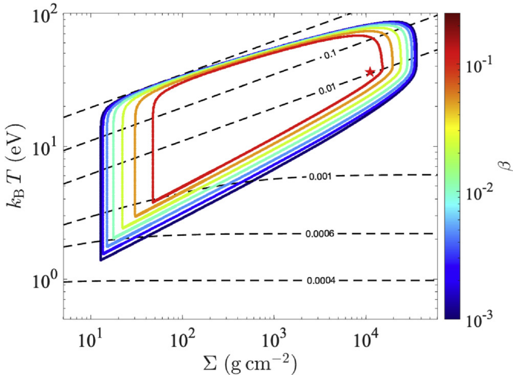
Figure 4. from Itai Linial and Brian D. Metzger 2024 Astrophys. J. 973 doi:10.3847/1538-4357/ad639e https://dx.doi.org/10.3847/1538-4357/ad639e © 2024. The Author(s). Published by the American Astronomical Society.
