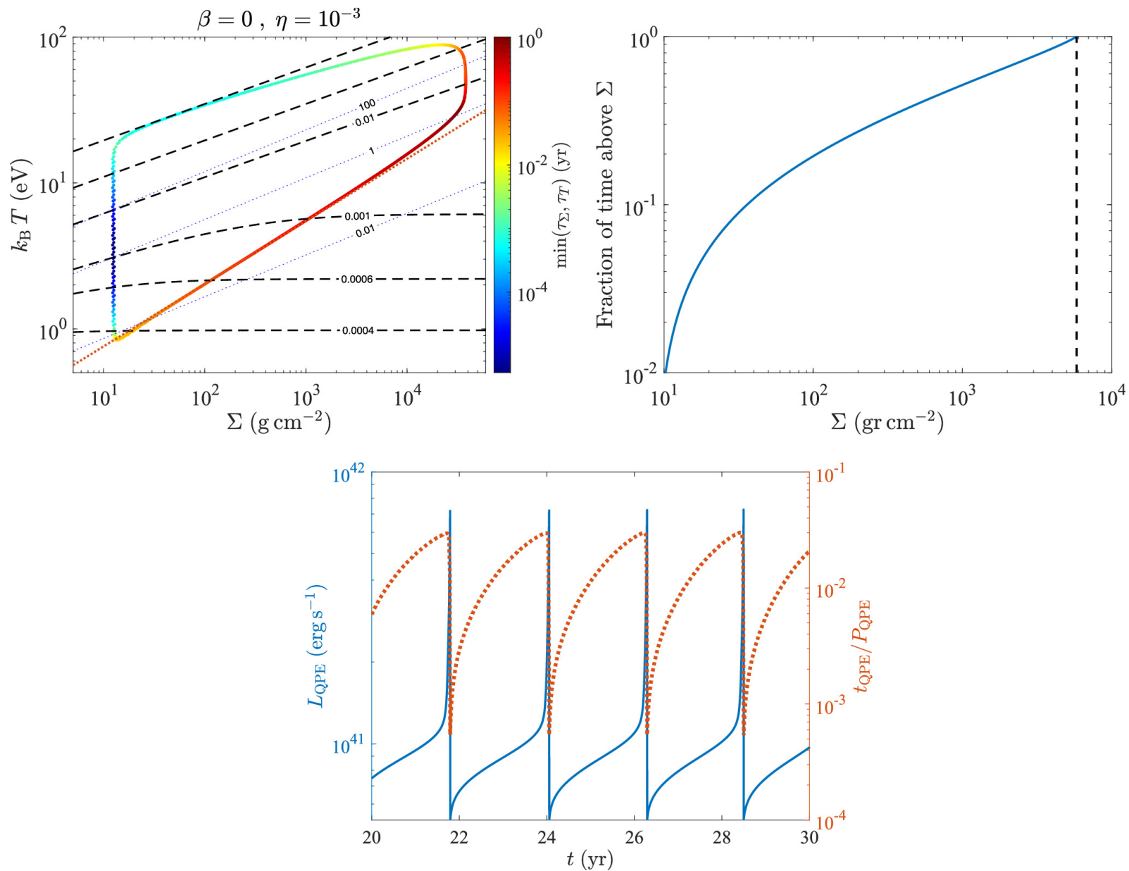
Figure 3. from Itai Linial and Brian D. Metzger 2024 Astrophys. J. 973 doi:10.3847/1538-4357/ad639e https://dx.doi.org/10.3847/1538-4357/ad639e © 2024. The Author(s). Published by the American Astronomical Society.
