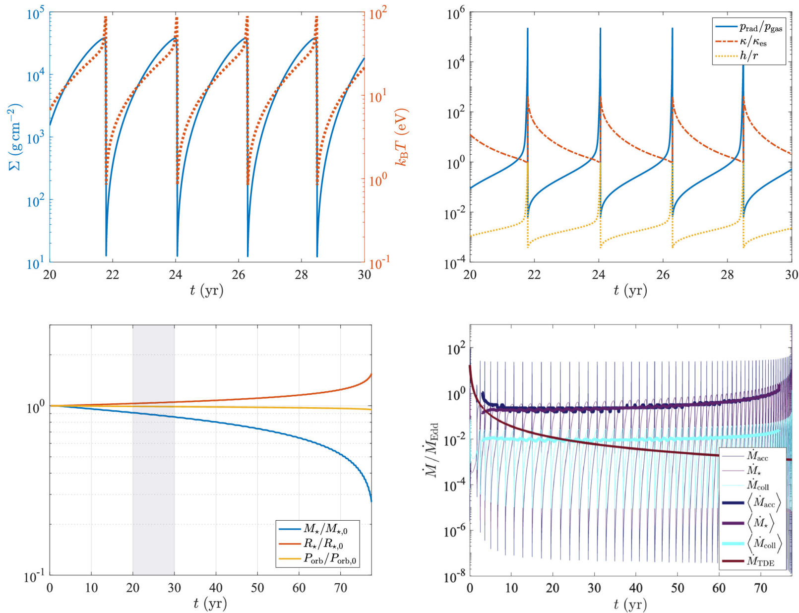
Figure 2. from Itai Linial and Brian D. Metzger 2024 Astrophys. J. 973 doi:10.3847/1538-4357/ad639e https://dx.doi.org/10.3847/1538-4357/ad639e © 2024. The Author(s). Published by the American Astronomical Society.
