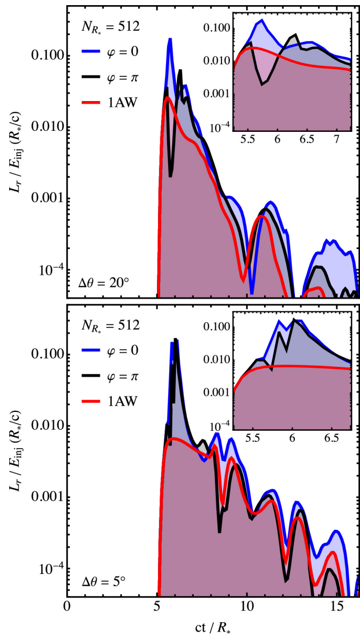
Figure 8. from Jens F. Mahlmann et al 2024 Astrophys. J. 972 doi:10.3847/1538-4357/ad60c4 https://dx.doi.org/10.3847/1538-4357/ad60c4 © 2024. The Author(s). Published by the American Astronomical Society.
