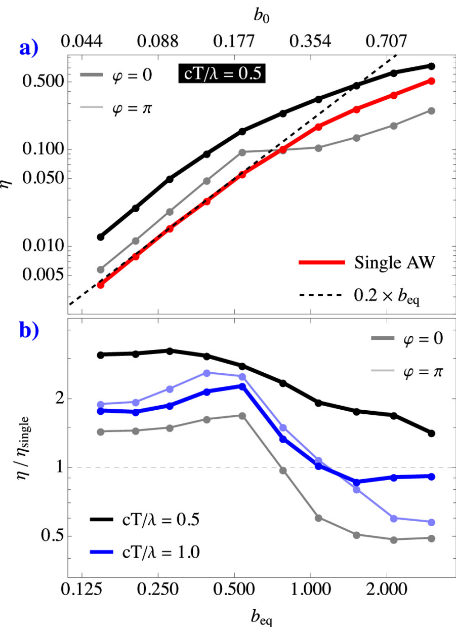
Figure 7. from Jens F. Mahlmann et al 2024 Astrophys. J. 972 doi:10.3847/1538-4357/ad60c4 https://dx.doi.org/10.3847/1538-4357/ad60c4 © 2024. The Author(s). Published by the American Astronomical Society.
