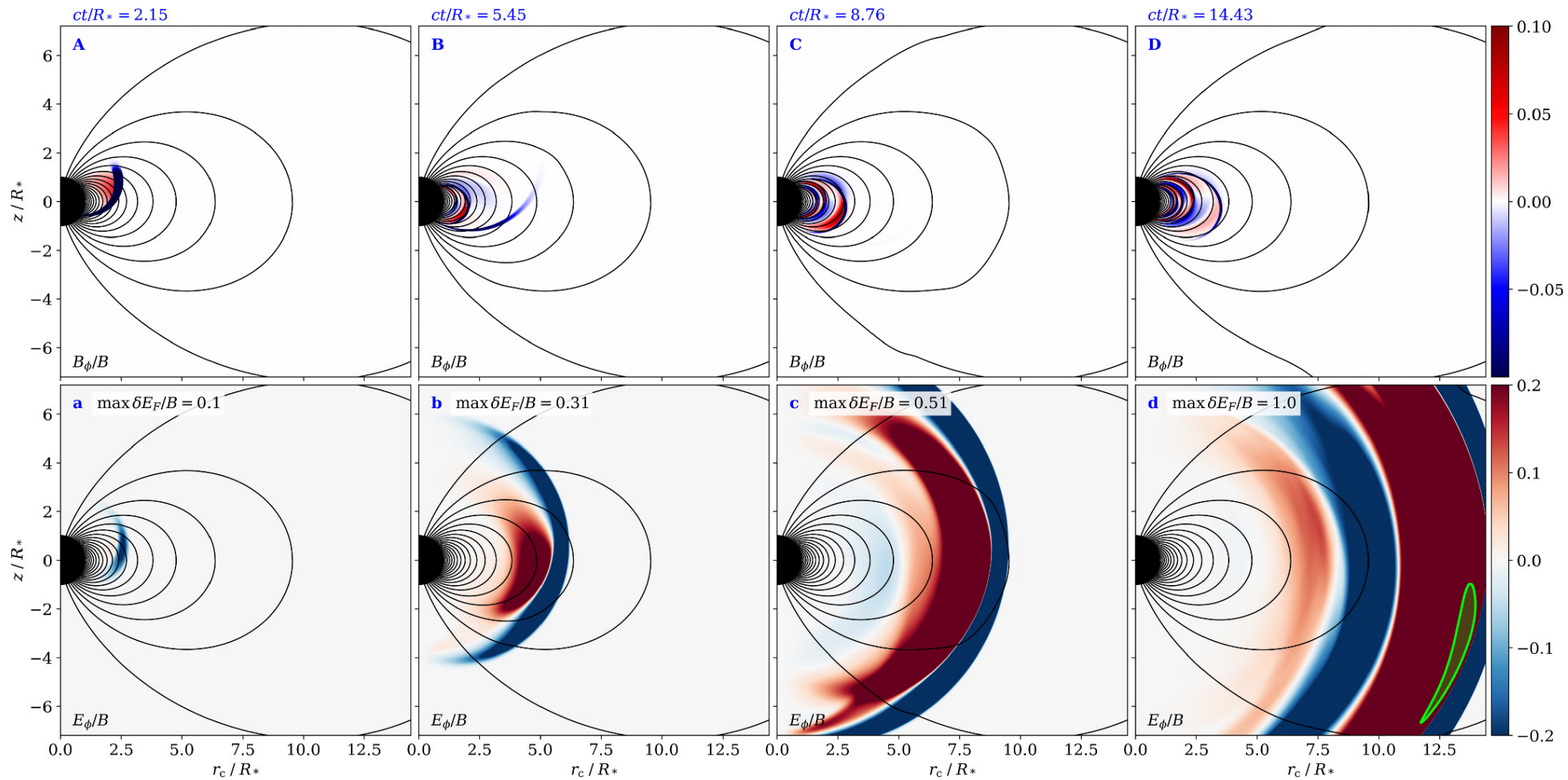
Figure 5. from Jens F. Mahlmann et al 2024 Astrophys. J. 972 doi:10.3847/1538-4357/ad60c4 https://dx.doi.org/10.3847/1538-4357/ad60c4 © 2024. The Author(s). Published by the American Astronomical Society.
