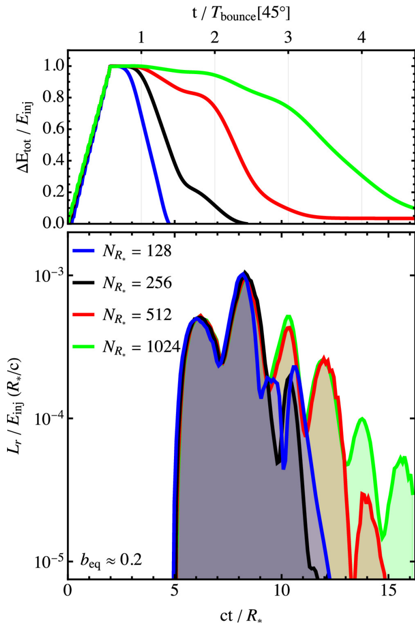
Figure 4. from Jens F. Mahlmann et al 2024 Astrophys. J. 972 doi:10.3847/1538-4357/ad60c4 https://dx.doi.org/10.3847/1538-4357/ad60c4 © 2024. The Author(s). Published by the American Astronomical Society.
