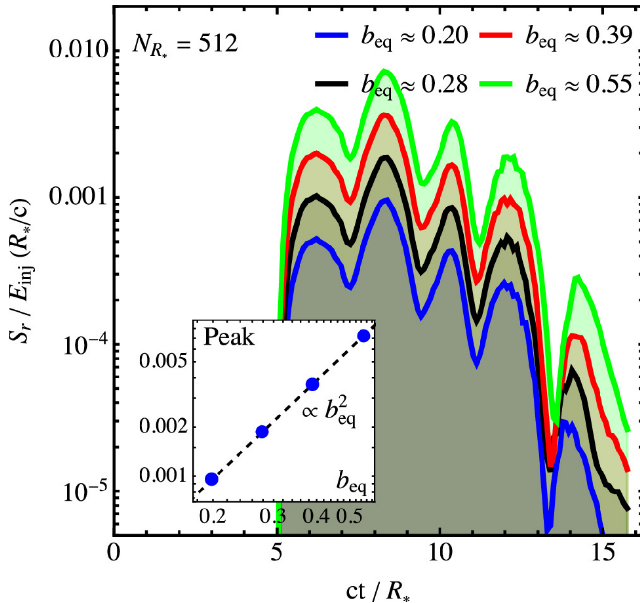
Figure 3. from Jens F. Mahlmann et al 2024 Astrophys. J. 972 doi:10.3847/1538-4357/ad60c4 https://dx.doi.org/10.3847/1538-4357/ad60c4 © 2024. The Author(s). Published by the American Astronomical Society.
