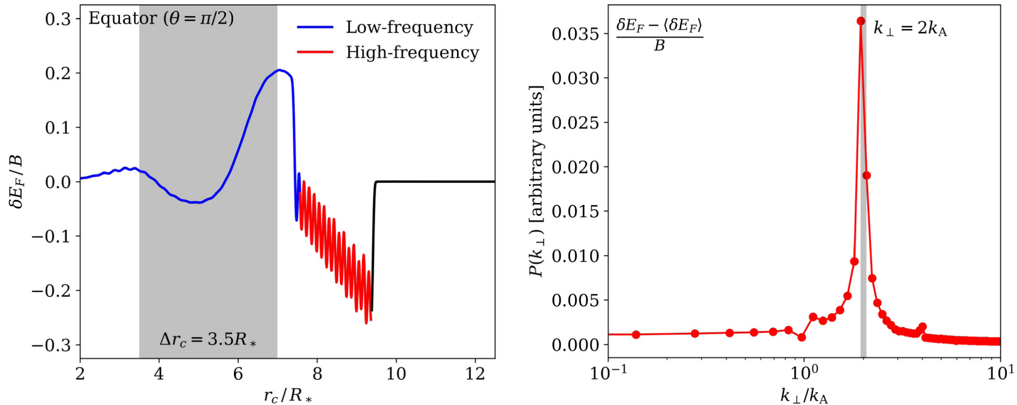
Figure 11. from Jens F. Mahlmann et al 2024 Astrophys. J. 972 doi:10.3847/1538-4357/ad60c4 https://dx.doi.org/10.3847/1538-4357/ad60c4 © 2024. The Author(s). Published by the American Astronomical Society.
