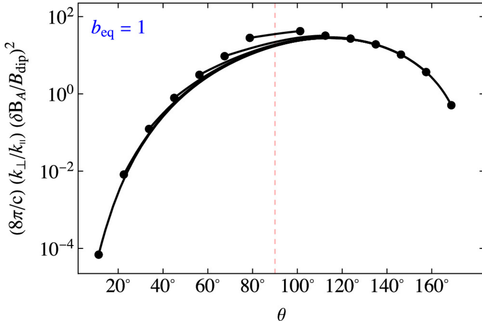
Figure 1. from Jens F. Mahlmann et al 2024 Astrophys. J. 972 doi:10.3847/1538-4357/ad60c4 https://dx.doi.org/10.3847/1538-4357/ad60c4 © 2024. The Author(s). Published by the American Astronomical Society.
