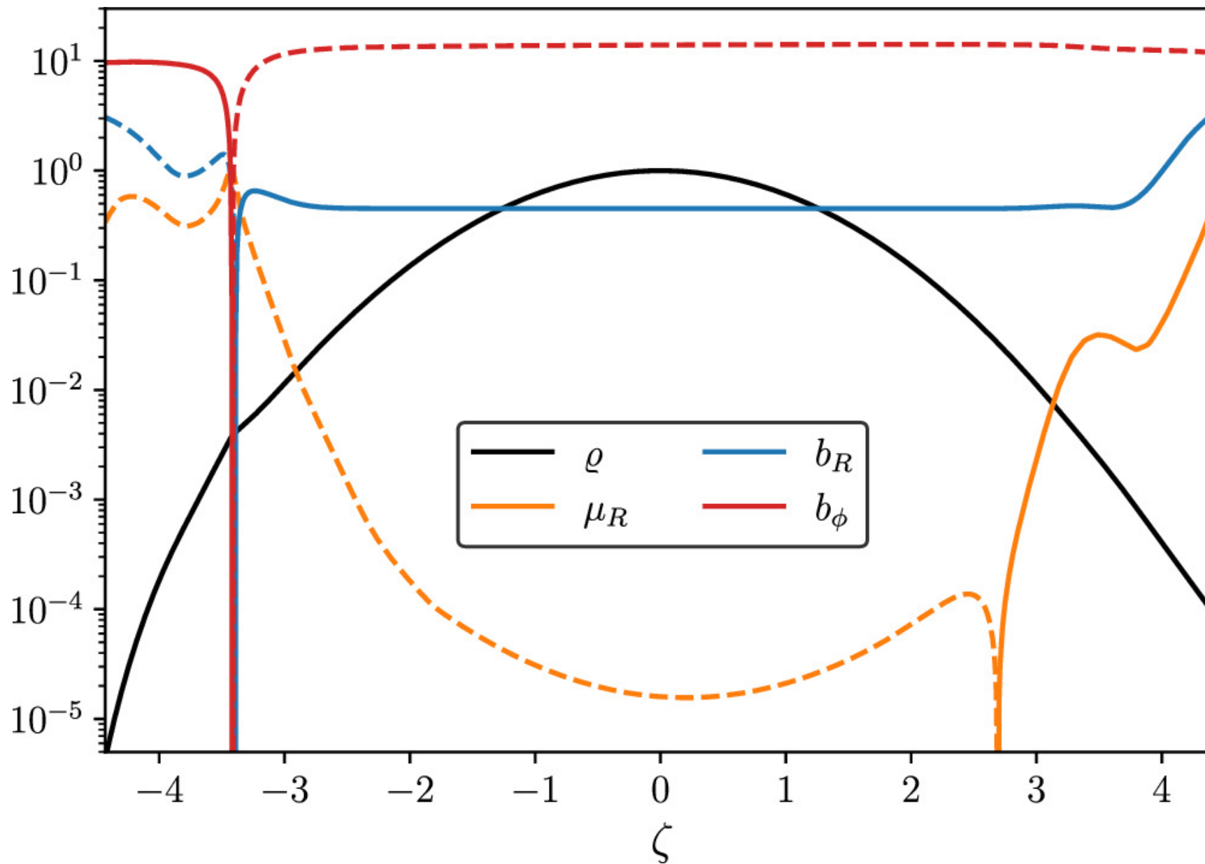
Figure 6. from Lile Wang et al 2024 Astrophys. J. 972 doi:10.3847/1538-4357/ad5f8d https://dx.doi.org/10.3847/1538-4357/ad5f8d © 2024. The Author(s). Published by the American Astronomical Society.
