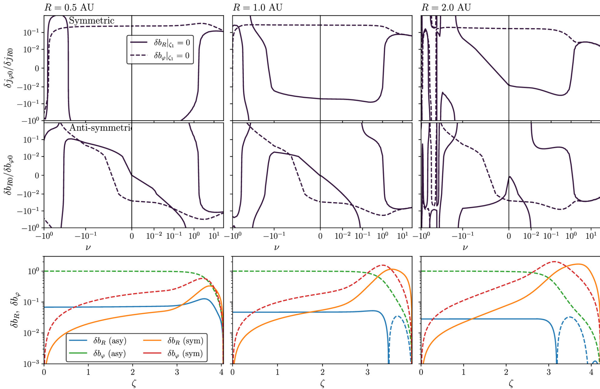
Figure 4. from Lile Wang et al 2024 Astrophys. J. 972 doi:10.3847/1538-4357/ad5f8d https://dx.doi.org/10.3847/1538-4357/ad5f8d © 2024. The Author(s). Published by the American Astronomical Society.
