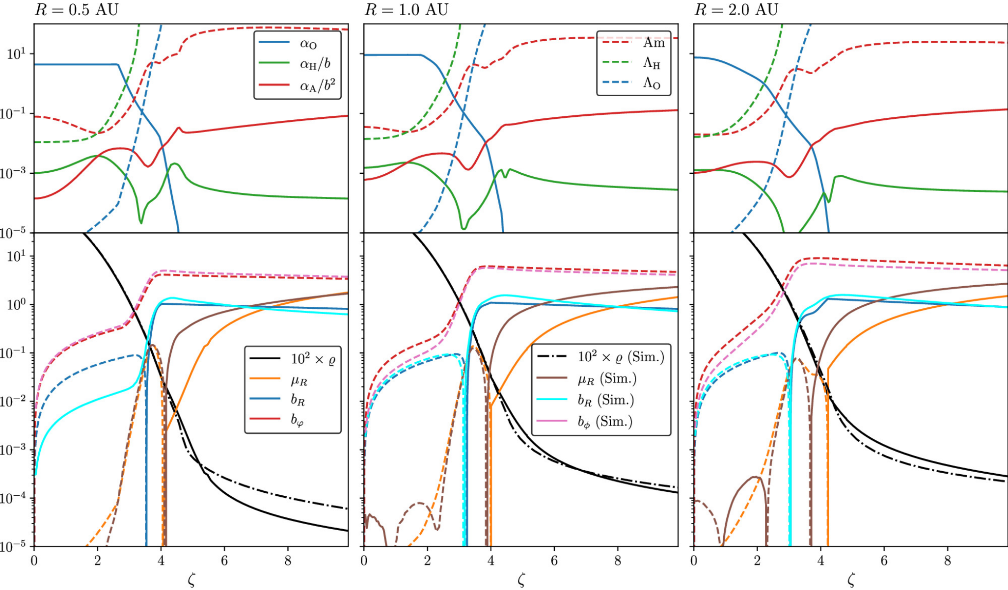
Figure 3. from Lile Wang et al 2024 Astrophys. J. 972 doi:10.3847/1538-4357/ad5f8d https://dx.doi.org/10.3847/1538-4357/ad5f8d © 2024. The Author(s). Published by the American Astronomical Society.
