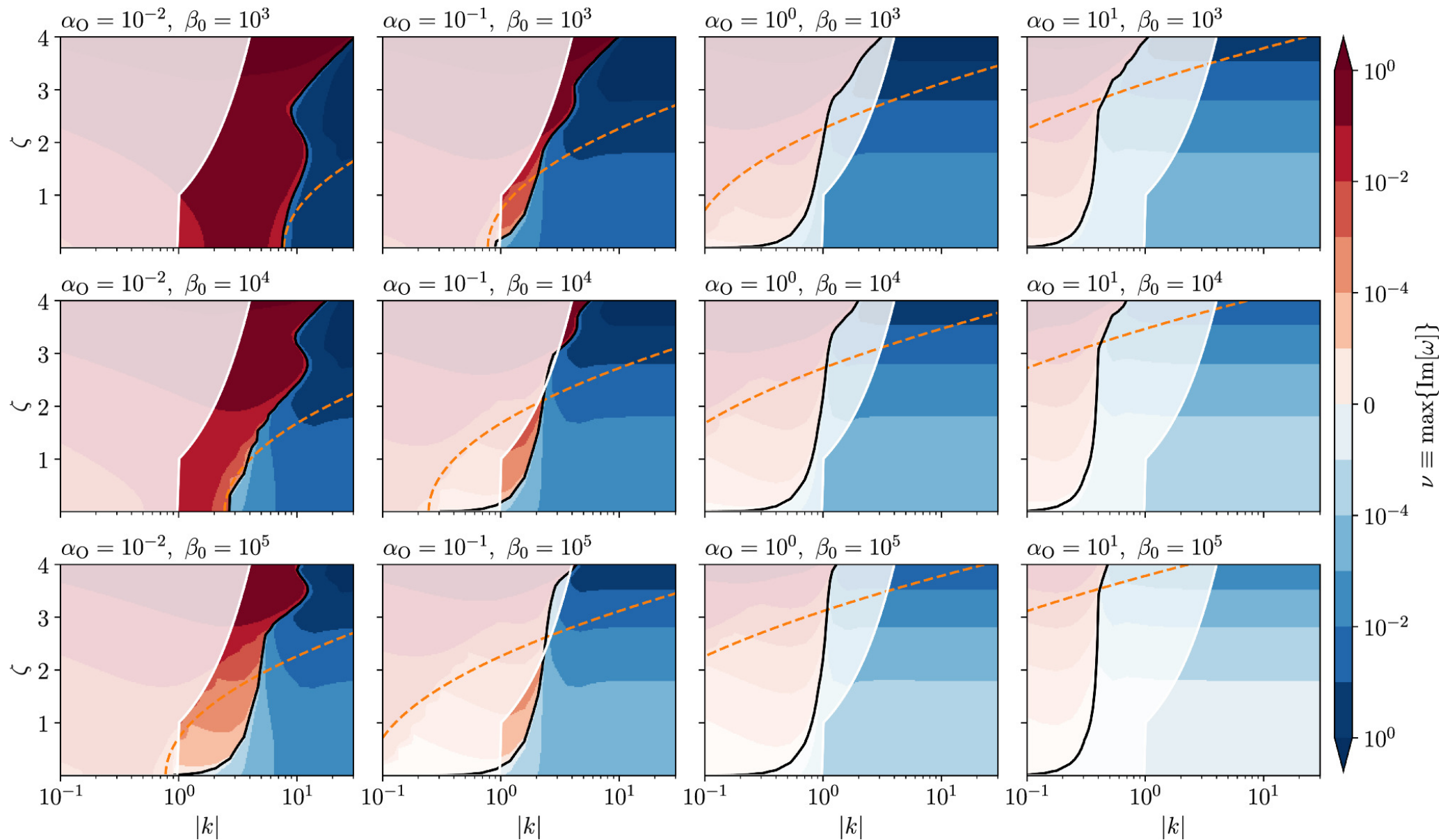
Figure 2. from Lile Wang et al 2024 Astrophys. J. 972 doi:10.3847/1538-4357/ad5f8d https://dx.doi.org/10.3847/1538-4357/ad5f8d © 2024. The Author(s). Published by the American Astronomical Society.
