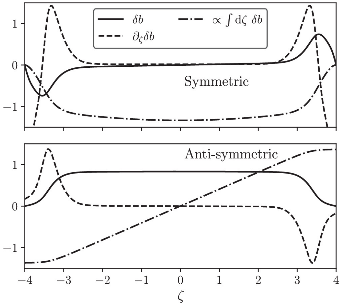
Figure 1. from Lile Wang et al 2024 Astrophys. J. 972 doi:10.3847/1538-4357/ad5f8d https://dx.doi.org/10.3847/1538-4357/ad5f8d © 2024. The Author(s). Published by the American Astronomical Society.
