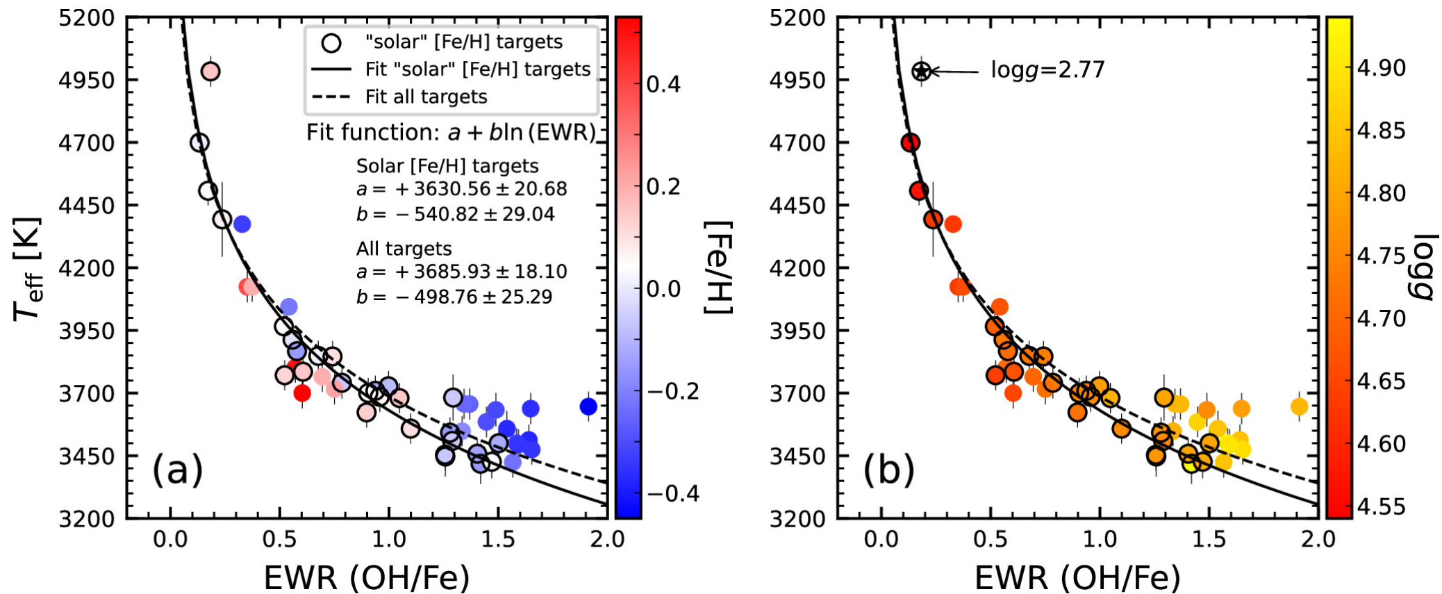
Figure 7. from Shih-Yun Tang et al 2024 Astrophys. J. 973 doi:10.3847/1538-4357/ad5e7f https://dx.doi.org/10.3847/1538-4357/ad5e7f © 2024. The Author(s). Published by the American Astronomical Society.
