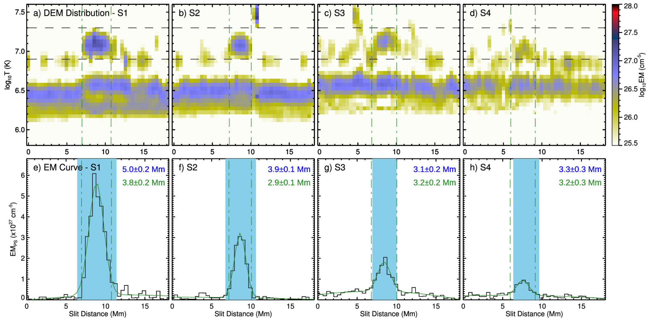
Figure 7. from Tingyu Gou and Katharine K. Reeves 2024 Astrophys. J. 972 doi:10.3847/1538-4357/ad5d61 https://dx.doi.org/10.3847/1538-4357/ad5d61 © 2024. The Author(s). Published by the American Astronomical Society.
