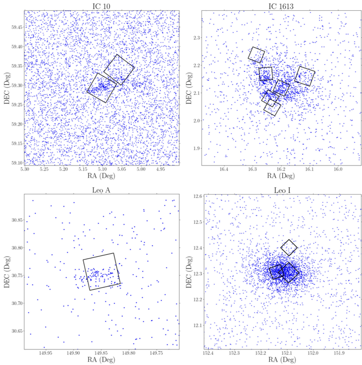
Figure A1. from Paul Bennet et al 2024 Astrophys. J. 971 doi:10.3847/1538-4357/ad5349 https://dx.doi.org/10.3847/1538-4357/ad5349 © 2024. The Author(s). Published by the American Astronomical Society.
