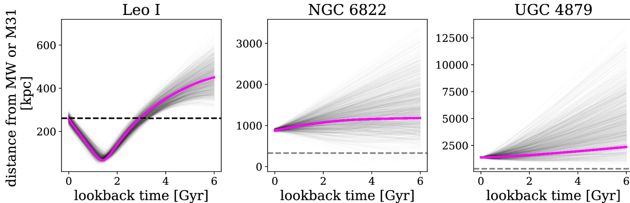
Figure 7. from Paul Bennet et al 2024 Astrophys. J. 971 doi:10.3847/1538-4357/ad5349 https://dx.doi.org/10.3847/1538-4357/ad5349 © 2024. The Author(s). Published by the American Astronomical Society.
