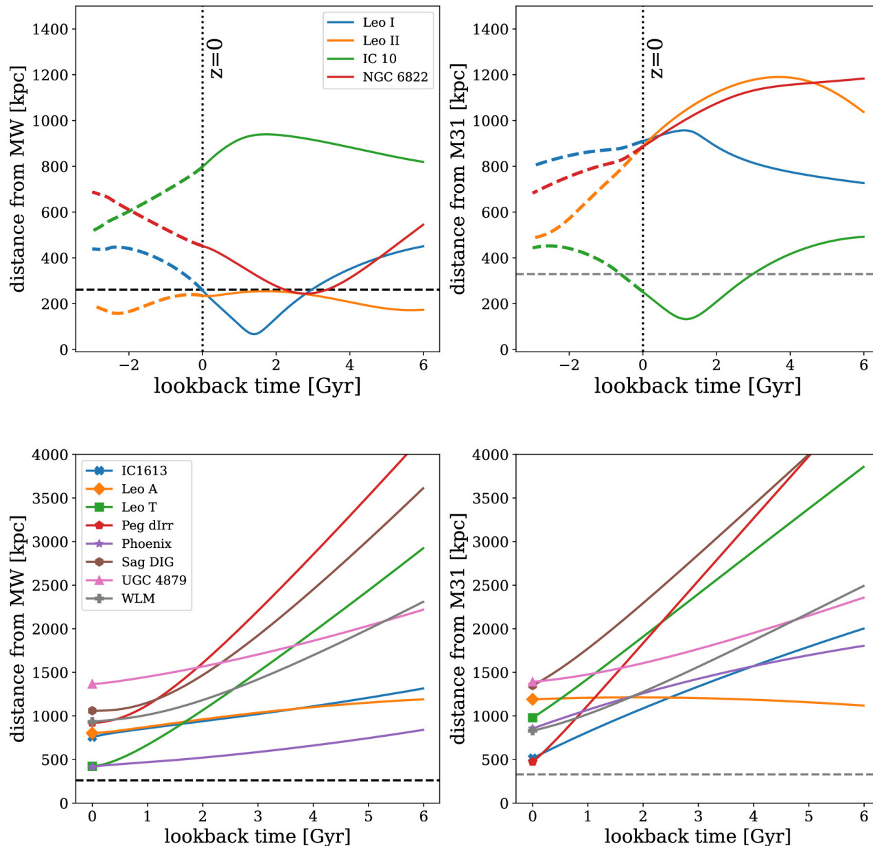
Figure 5. from Paul Bennet et al 2024 Astrophys. J. 971 doi:10.3847/1538-4357/ad5349 https://dx.doi.org/10.3847/1538-4357/ad5349 © 2024. The Author(s). Published by the American Astronomical Society.
