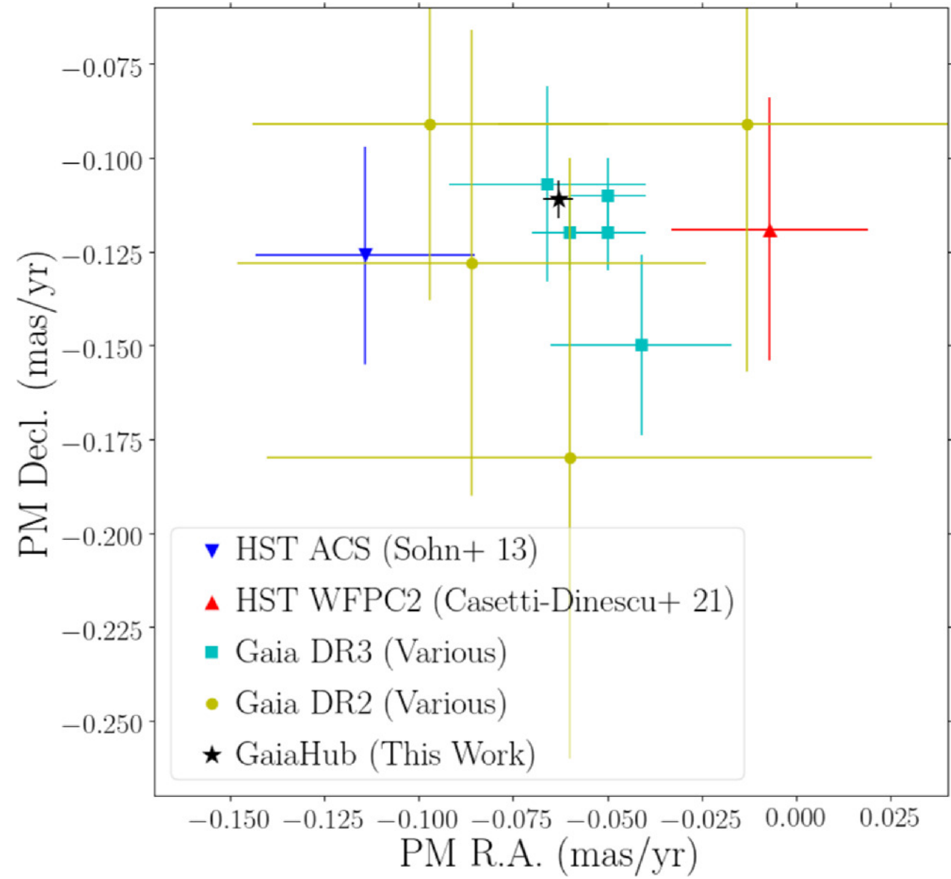
Figure 4. from Paul Bennet et al 2024 Astrophys. J. 971 doi:10.3847/1538-4357/ad5349 https://dx.doi.org/10.3847/1538-4357/ad5349 © 2024. The Author(s). Published by the American Astronomical Society.
