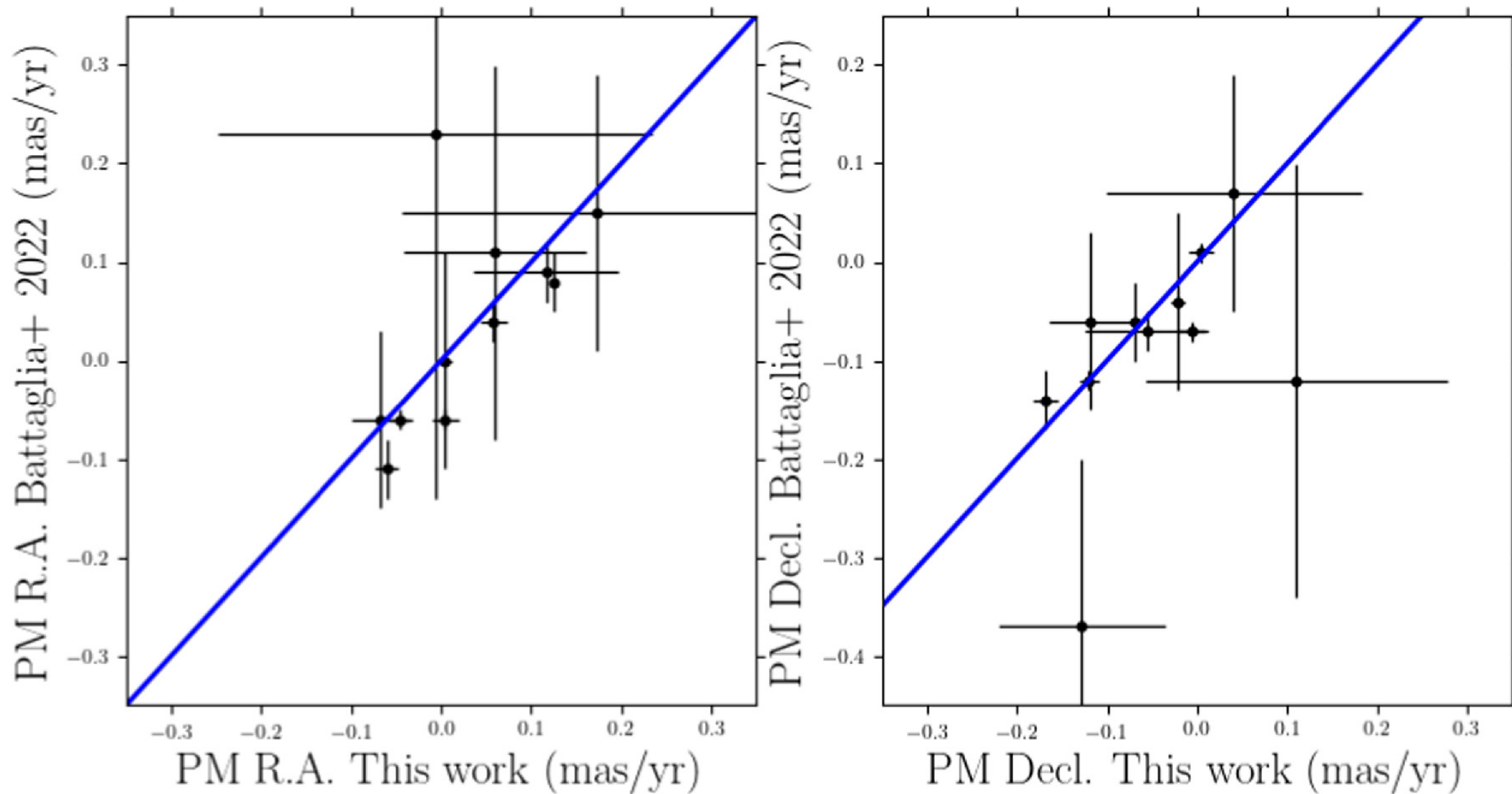
Figure 3. from Paul Bennet et al 2024 Astrophys. J. 971 doi:10.3847/1538-4357/ad5349 https://dx.doi.org/10.3847/1538-4357/ad5349 © 2024. The Author(s). Published by the American Astronomical Society.
