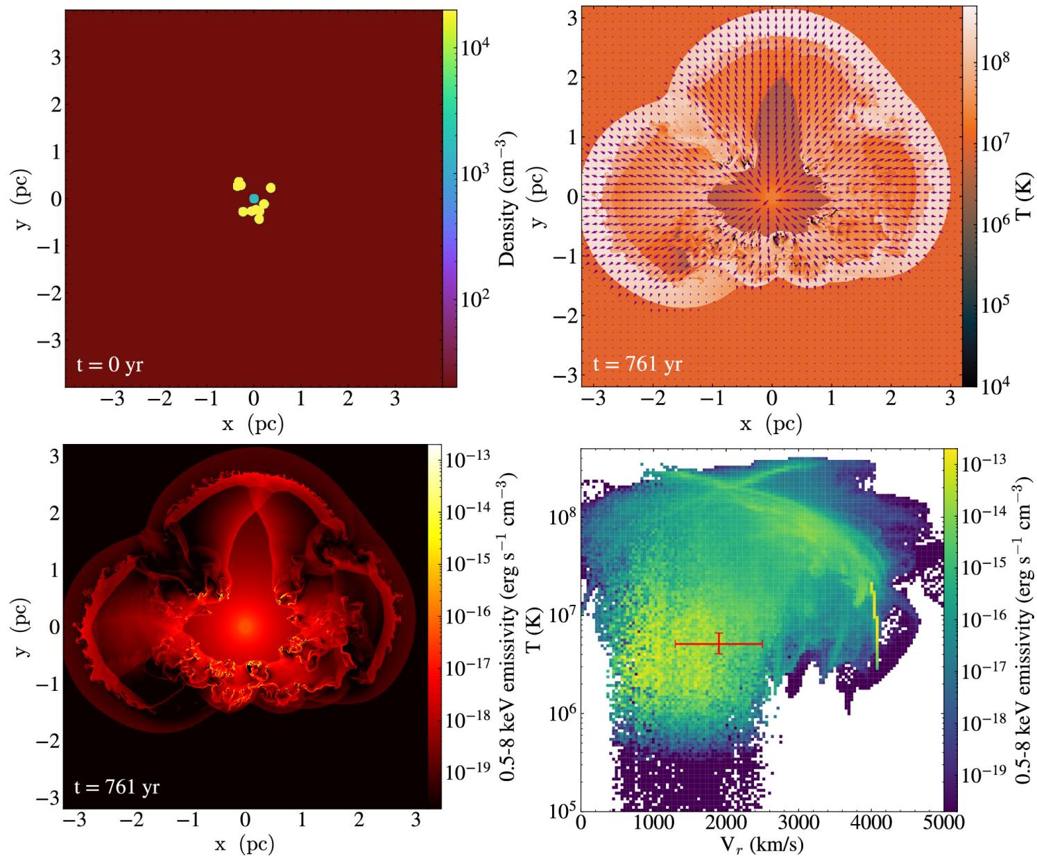
Figure D1. from Fangzheng Shi et al 2024 Astrophys. J. 970 doi:10.3847/1538-4357/ad4ed7 https://dx.doi.org/10.3847/1538-4357/ad4ed7 © 2024. The Author(s). Published by the American Astronomical Society.
