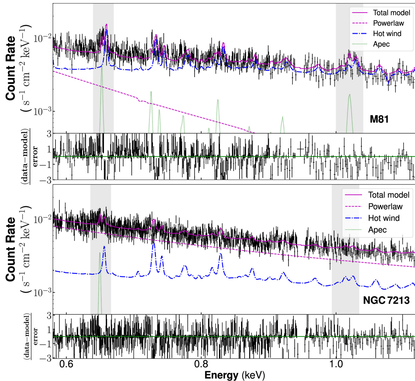
Figure C1. from Fangzheng Shi et al 2024 Astrophys. J. 970 doi:10.3847/1538-4357/ad4ed7 https://dx.doi.org/10.3847/1538-4357/ad4ed7 © 2024. The Author(s). Published by the American Astronomical Society.
