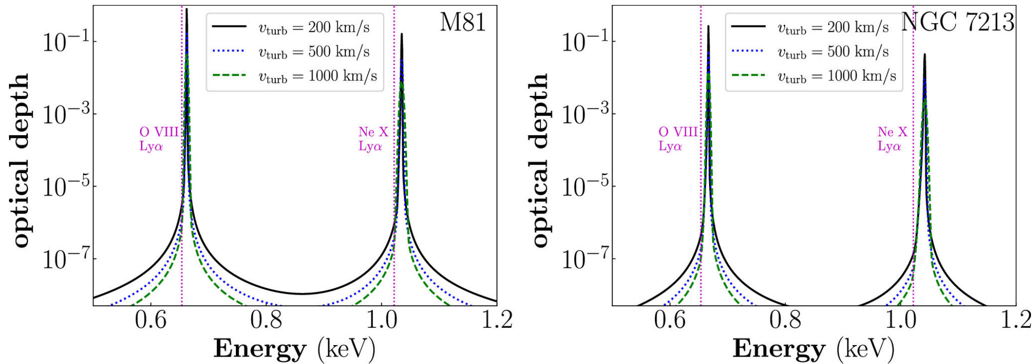
Figure B1. from Fangzheng Shi et al 2024 Astrophys. J. 970 doi:10.3847/1538-4357/ad4ed7 https://dx.doi.org/10.3847/1538-4357/ad4ed7 © 2024. The Author(s). Published by the American Astronomical Society.
