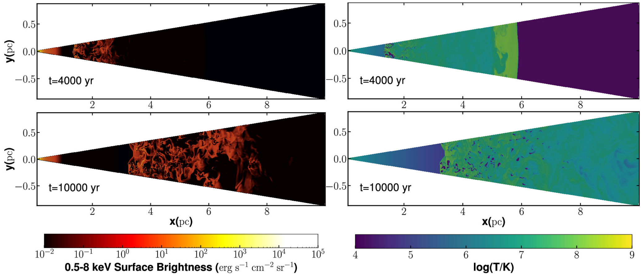
Figure 4. from Fangzheng Shi et al 2024 Astrophys. J. 970 doi:10.3847/1538-4357/ad4ed7 https://dx.doi.org/10.3847/1538-4357/ad4ed7 © 2024. The Author(s). Published by the American Astronomical Society.
