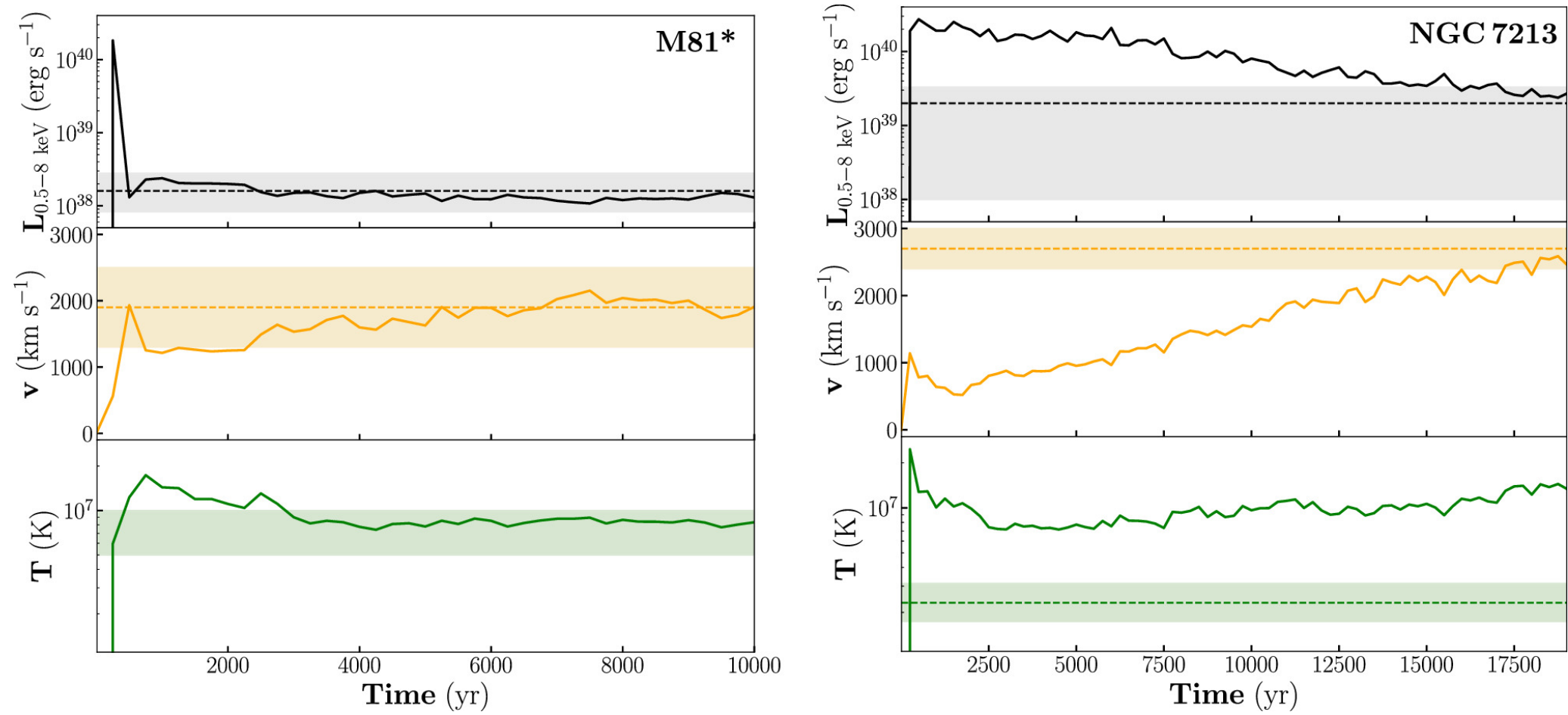
Figure 3. from Fangzheng Shi et al 2024 Astrophys. J. 970 doi:10.3847/1538-4357/ad4ed7 https://dx.doi.org/10.3847/1538-4357/ad4ed7 © 2024. The Author(s). Published by the American Astronomical Society.
