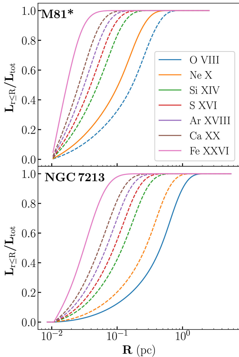
Figure 2. from Fangzheng Shi et al 2024 Astrophys. J. 970 doi:10.3847/1538-4357/ad4ed7 https://dx.doi.org/10.3847/1538-4357/ad4ed7 © 2024. The Author(s). Published by the American Astronomical Society.
