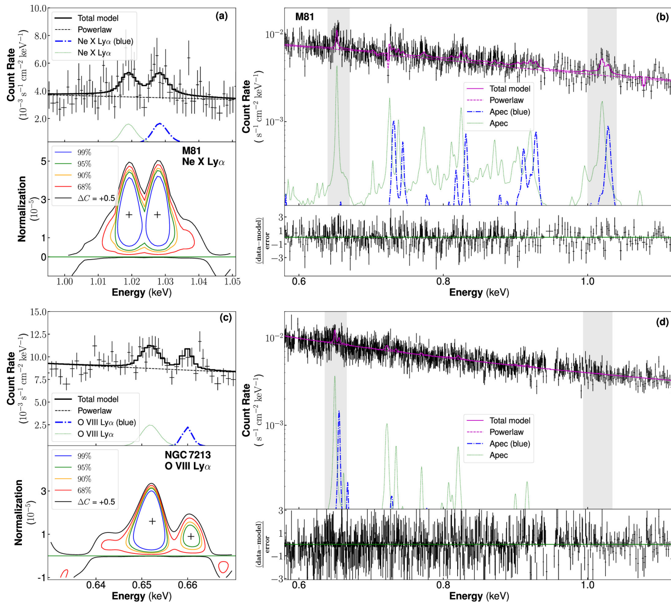
Figure 1. from Fangzheng Shi et al 2024 Astrophys. J. 970 doi:10.3847/1538-4357/ad4ed7 https://dx.doi.org/10.3847/1538-4357/ad4ed7 © 2024. The Author(s). Published by the American Astronomical Society.
