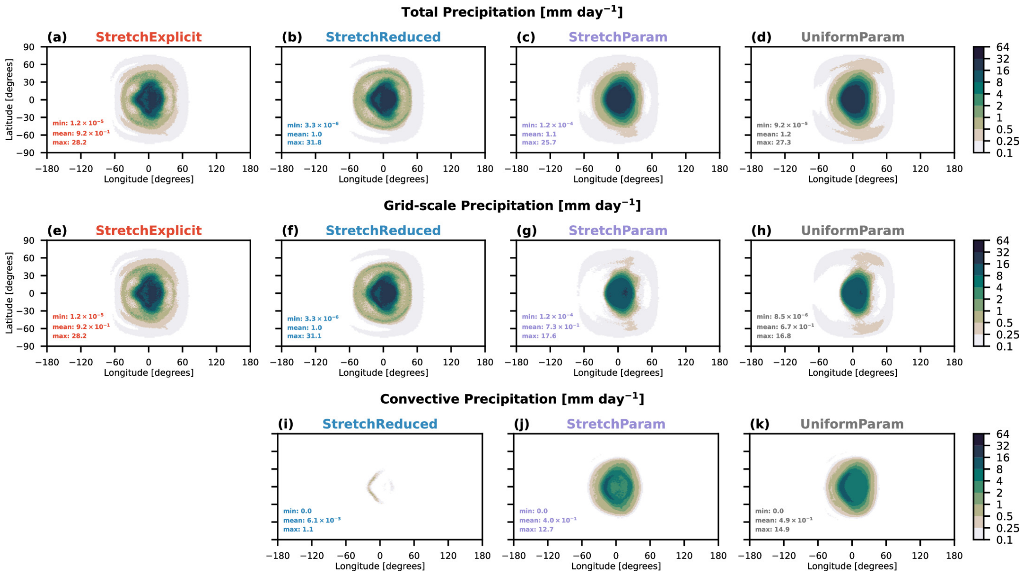
Figure 6. from Denis E. Sergeev et al 2024 Astrophys. J. 970 doi:10.3847/1538-4357/ad4ecd https://dx.doi.org/10.3847/1538-4357/ad4ecd © 2024. The Author(s). Published by the American Astronomical Society.
