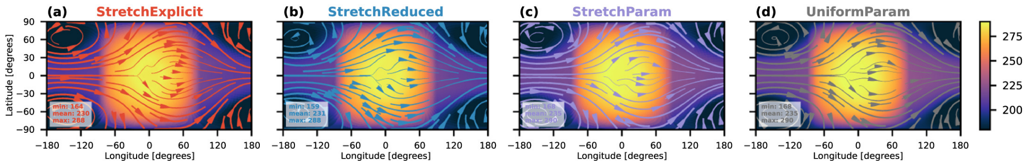
Figure 5. from Denis E. Sergeev et al 2024 Astrophys. J. 970 doi:10.3847/1538-4357/ad4ecd https://dx.doi.org/10.3847/1538-4357/ad4ecd © 2024. The Author(s). Published by the American Astronomical Society.
