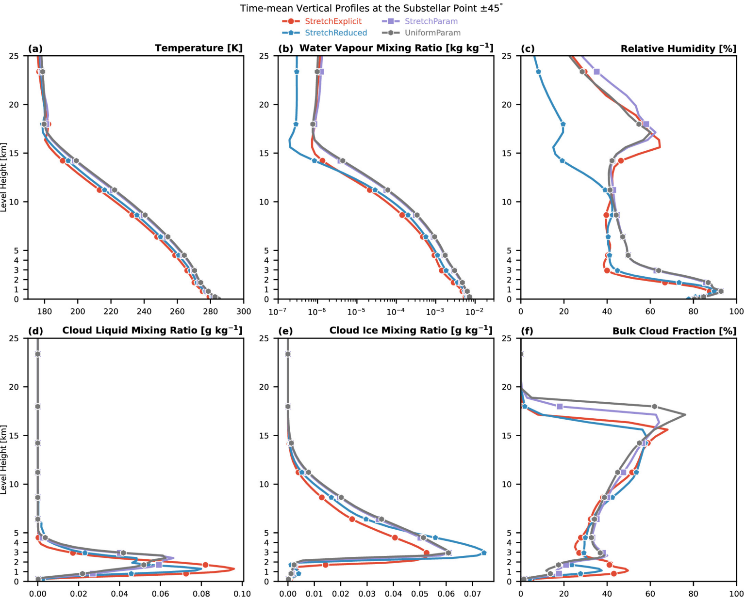
Figure 4. from Denis E. Sergeev et al 2024 Astrophys. J. 970 doi:10.3847/1538-4357/ad4ecd https://dx.doi.org/10.3847/1538-4357/ad4ecd © 2024. The Author(s). Published by the American Astronomical Society.
