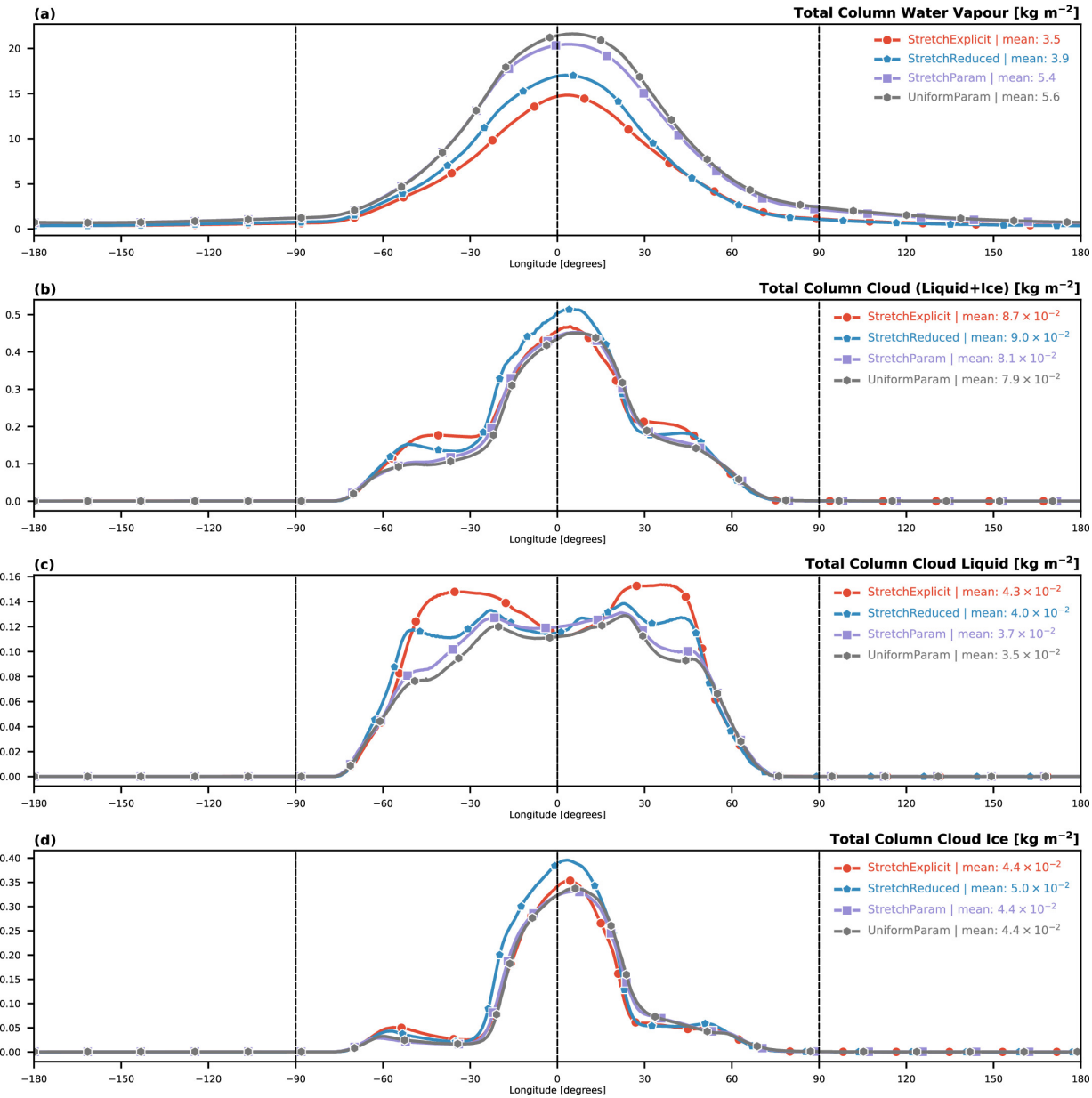
Figure 3. from Denis E. Sergeev et al 2024 Astrophys. J. 970 doi:10.3847/1538-4357/ad4ecd https://dx.doi.org/10.3847/1538-4357/ad4ecd © 2024. The Author(s). Published by the American Astronomical Society.
