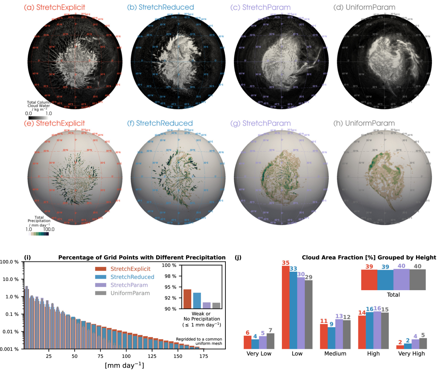
Figure 2. from Denis E. Sergeev et al 2024 Astrophys. J. 970 doi:10.3847/1538-4357/ad4ecd https://dx.doi.org/10.3847/1538-4357/ad4ecd © 2024. The Author(s). Published by the American Astronomical Society.
