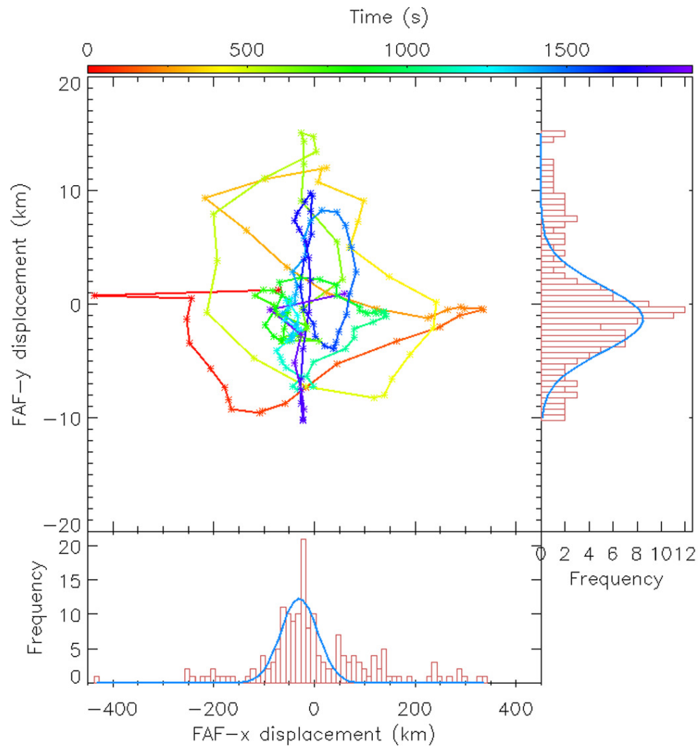
Figure 9. from W. Bate et al 2024 Astrophys. J. 970 doi:10.3847/1538-4357/ad4d97 https://dx.doi.org/10.3847/1538-4357/ad4d97 © 2024. The Author(s). Published by the American Astronomical Society.
