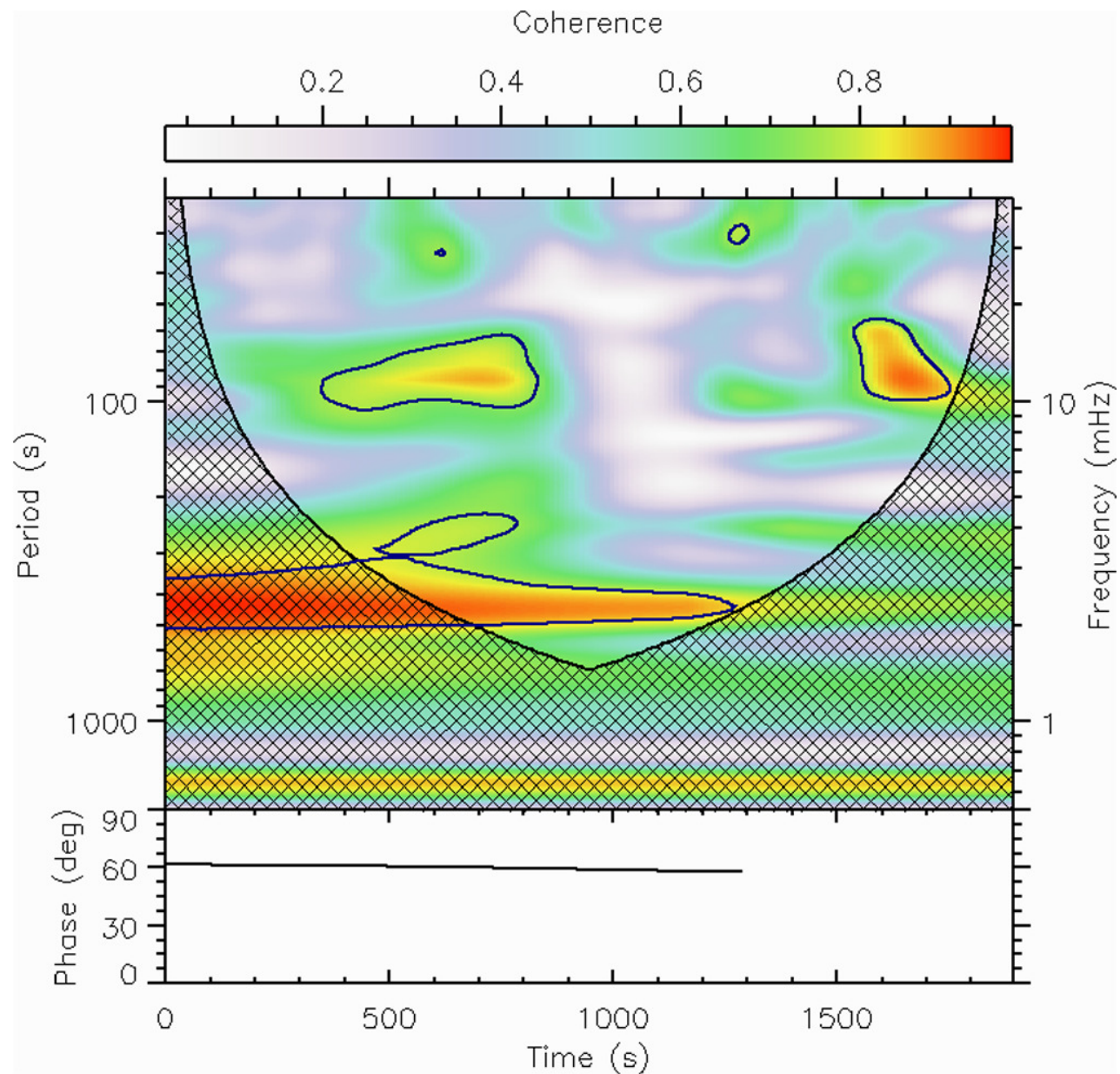
Figure 8. from W. Bate et al 2024 Astrophys. J. 970 doi:10.3847/1538-4357/ad4d97 https://dx.doi.org/10.3847/1538-4357/ad4d97 © 2024. The Author(s). Published by the American Astronomical Society.
