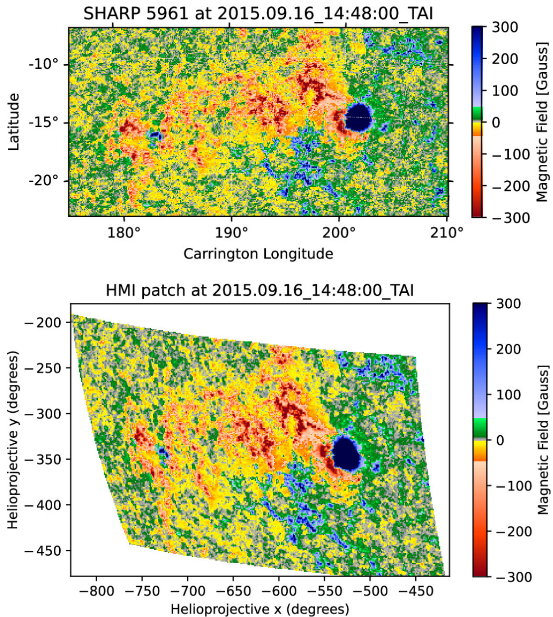
Figure 4. from W. Bate et al 2024 Astrophys. J. 970 doi:10.3847/1538-4357/ad4d97 https://dx.doi.org/10.3847/1538-4357/ad4d97 © 2024. The Author(s). Published by the American Astronomical Society.
