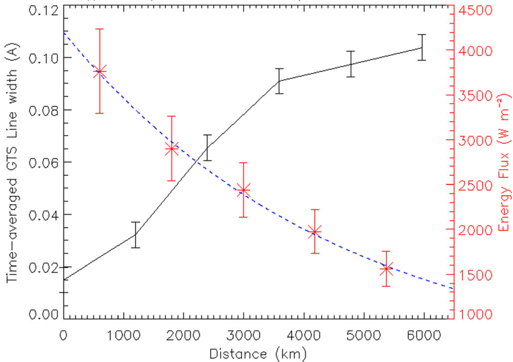
Figure 13. from W. Bate et al 2024 Astrophys. J. 970 doi:10.3847/1538-4357/ad4d97 https://dx.doi.org/10.3847/1538-4357/ad4d97 © 2024. The Author(s). Published by the American Astronomical Society.
