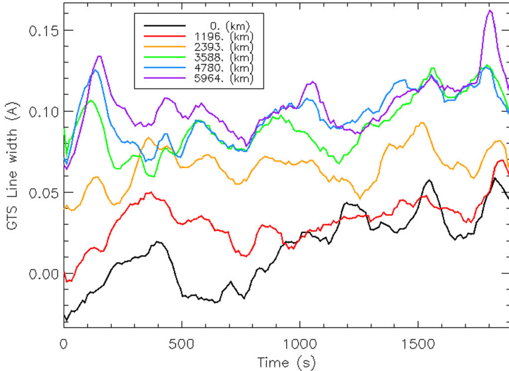
Figure 11. from W. Bate et al 2024 Astrophys. J. 970 doi:10.3847/1538-4357/ad4d97 https://dx.doi.org/10.3847/1538-4357/ad4d97 © 2024. The Author(s). Published by the American Astronomical Society.
