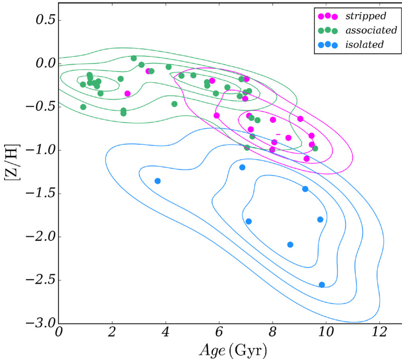
Figure 6. from J. K. Jang et al 2024 Astrophys. J. 969 doi:10.3847/1538-4357/ad4d8a https://dx.doi.org/10.3847/1538-4357/ad4d8a © 2024. The Author(s). Published by the American Astronomical Society.
