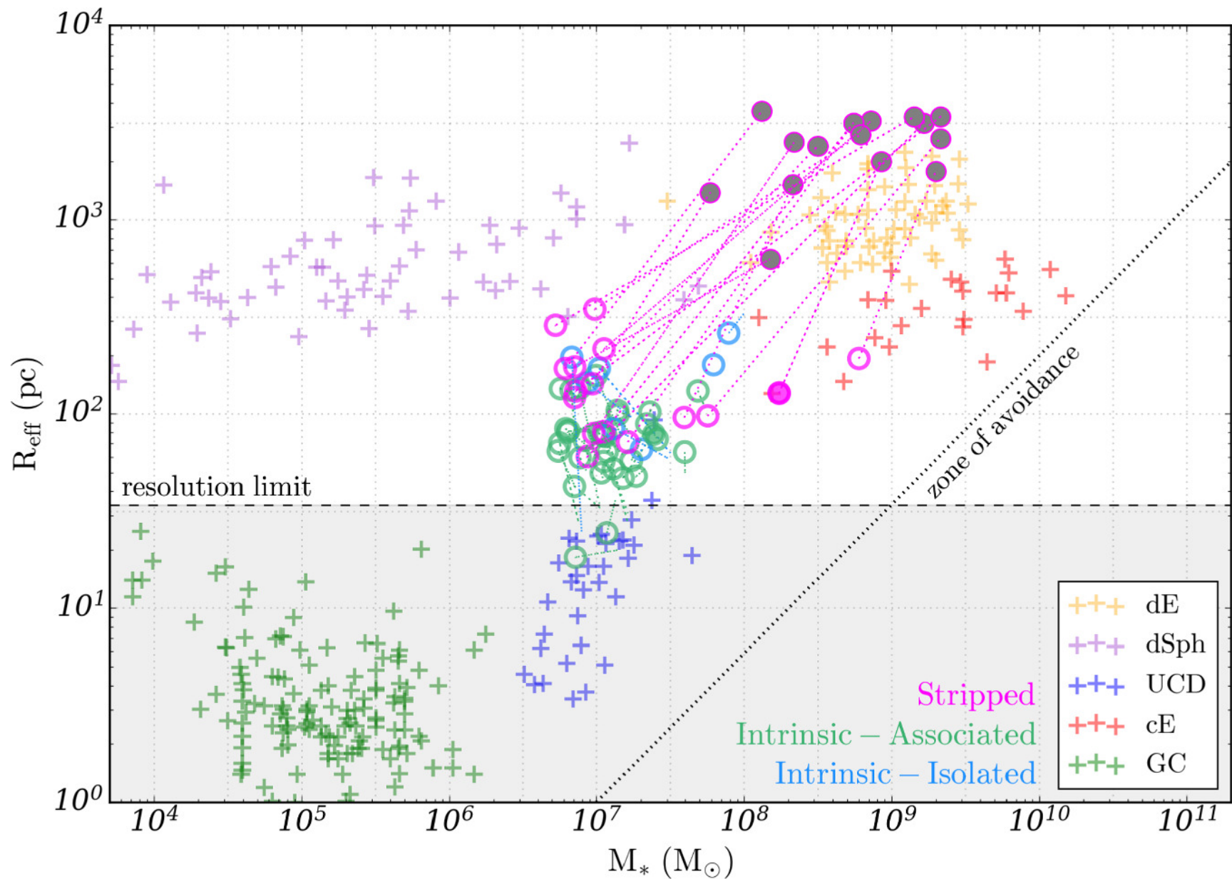
Figure 4. from J. K. Jang et al 2024 Astrophys. J. 969 doi:10.3847/1538-4357/ad4d8a https://dx.doi.org/10.3847/1538-4357/ad4d8a © 2024. The Author(s). Published by the American Astronomical Society.
