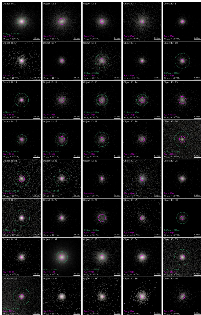
Figure 1. from J. K. Jang et al 2024 Astrophys. J. 969 doi:10.3847/1538-4357/ad4d8a https://dx.doi.org/10.3847/1538-4357/ad4d8a © 2024. The Author(s). Published by the American Astronomical Society.
