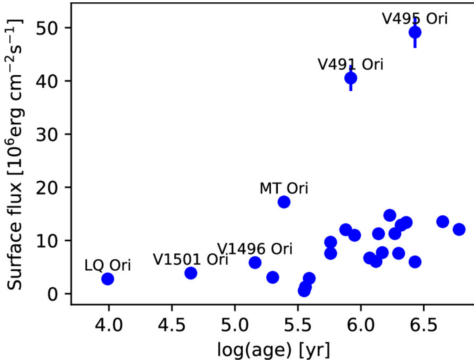
Figure 8. from Norbert S. Schulz et al 2024 Astrophys. J. 970 doi:10.3847/1538-4357/ad47c2 https://dx.doi.org/10.3847/1538-4357/ad47c2 © 2024. The Author(s). Published by the American Astronomical Society.
