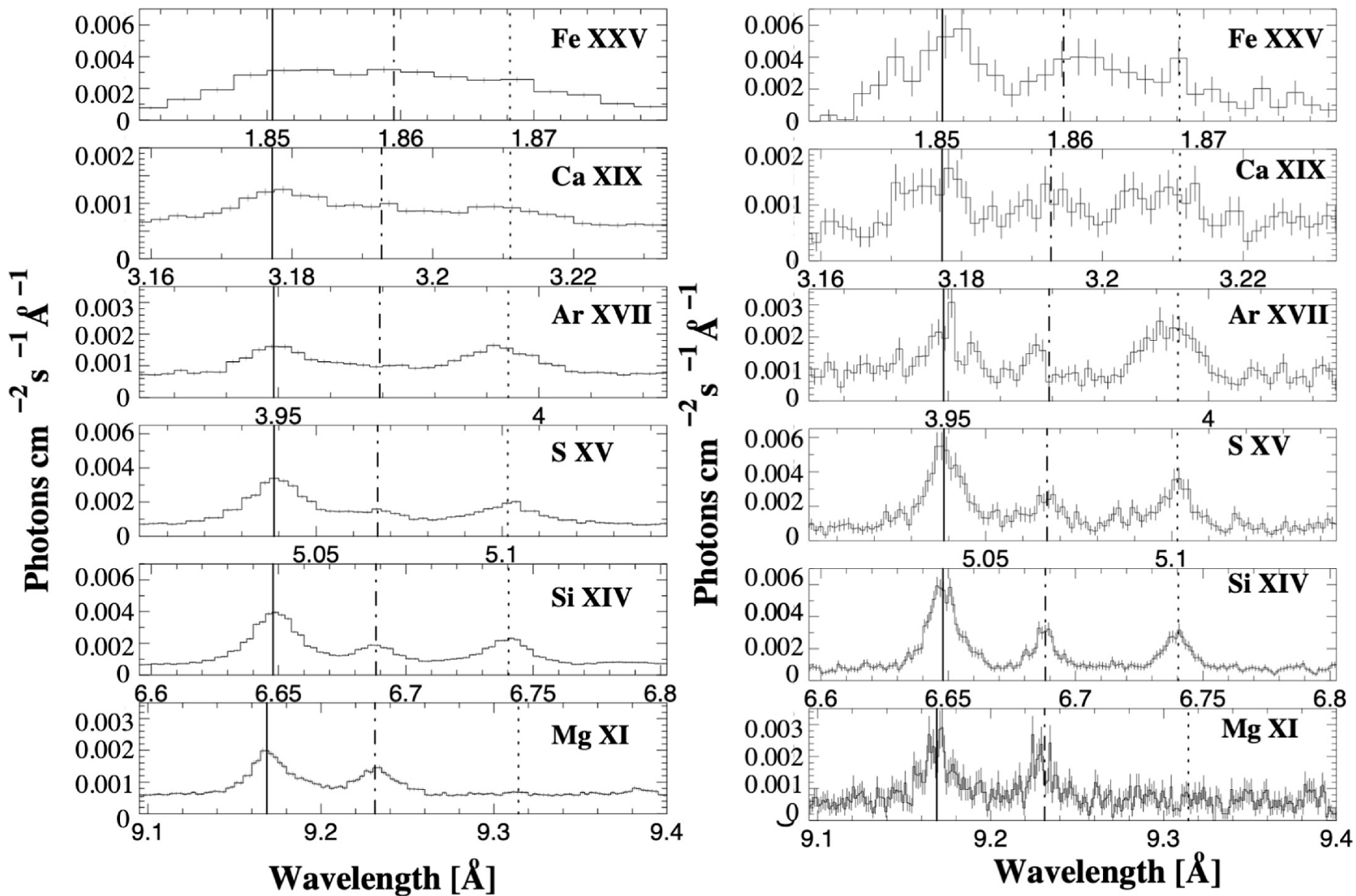
Figure 7. from Norbert S. Schulz et al 2024 Astrophys. J. 970 doi:10.3847/1538-4357/ad47c2 https://dx.doi.org/10.3847/1538-4357/ad47c2 © 2024. The Author(s). Published by the American Astronomical Society.
