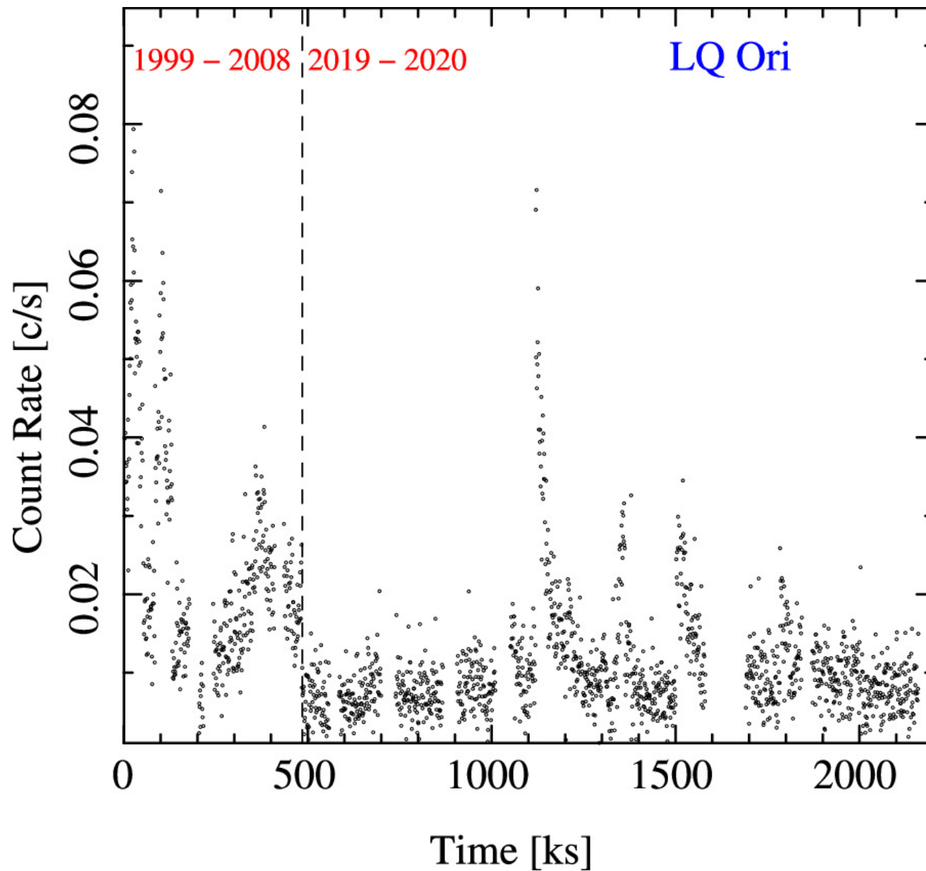
Figure 4. from Norbert S. Schulz et al 2024 Astrophys. J. 970 doi:10.3847/1538-4357/ad47c2 https://dx.doi.org/10.3847/1538-4357/ad47c2 © 2024. The Author(s). Published by the American Astronomical Society.
