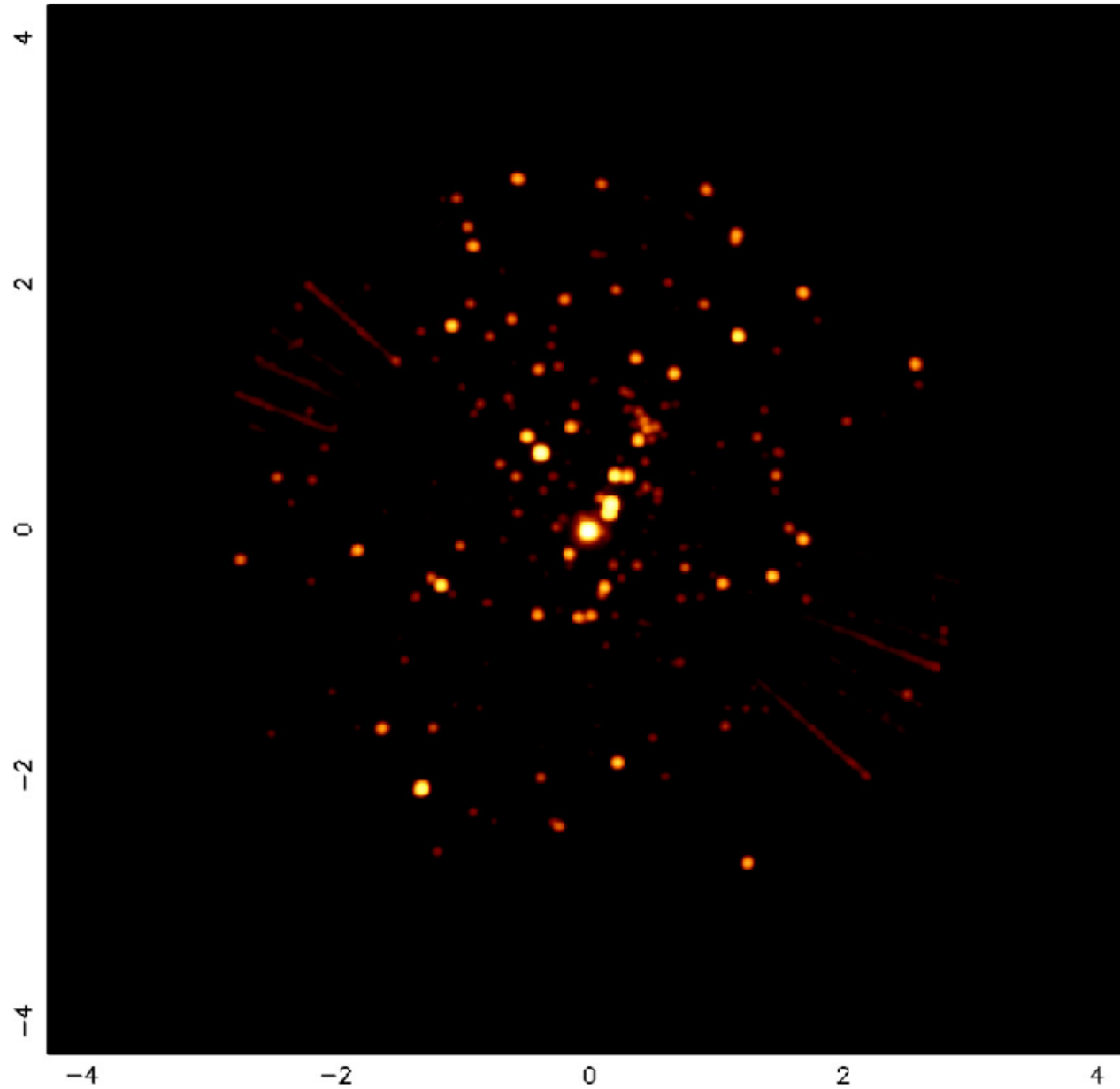
Figure 3. from Norbert S. Schulz et al 2024 Astrophys. J. 970 doi:10.3847/1538-4357/ad47c2 https://dx.doi.org/10.3847/1538-4357/ad47c2 © 2024. The Author(s). Published by the American Astronomical Society.
