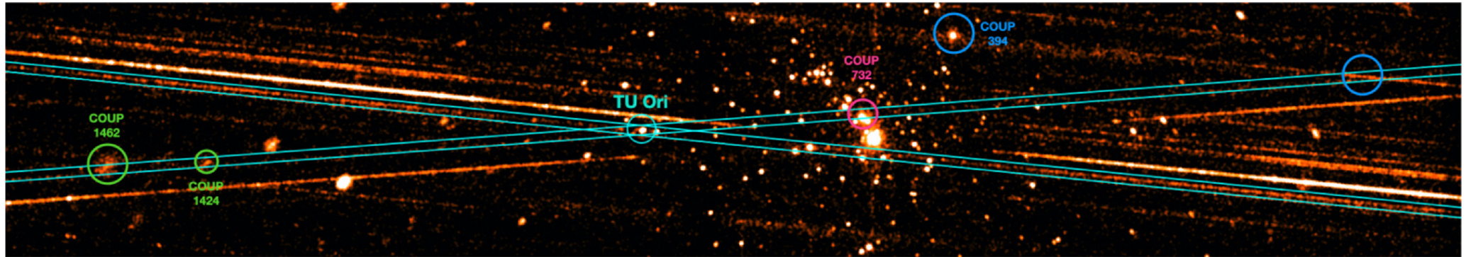
Figure 2. from Norbert S. Schulz et al 2024 Astrophys. J. 970 doi:10.3847/1538-4357/ad47c2 https://dx.doi.org/10.3847/1538-4357/ad47c2 © 2024. The Author(s). Published by the American Astronomical Society.
