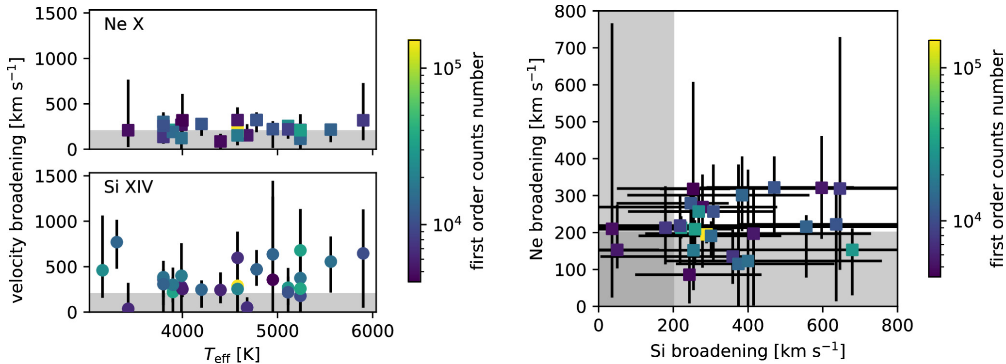
Figure 12. from Norbert S. Schulz et al 2024 Astrophys. J. 970 doi:10.3847/1538-4357/ad47c2 https://dx.doi.org/10.3847/1538-4357/ad47c2 © 2024. The Author(s). Published by the American Astronomical Society.
